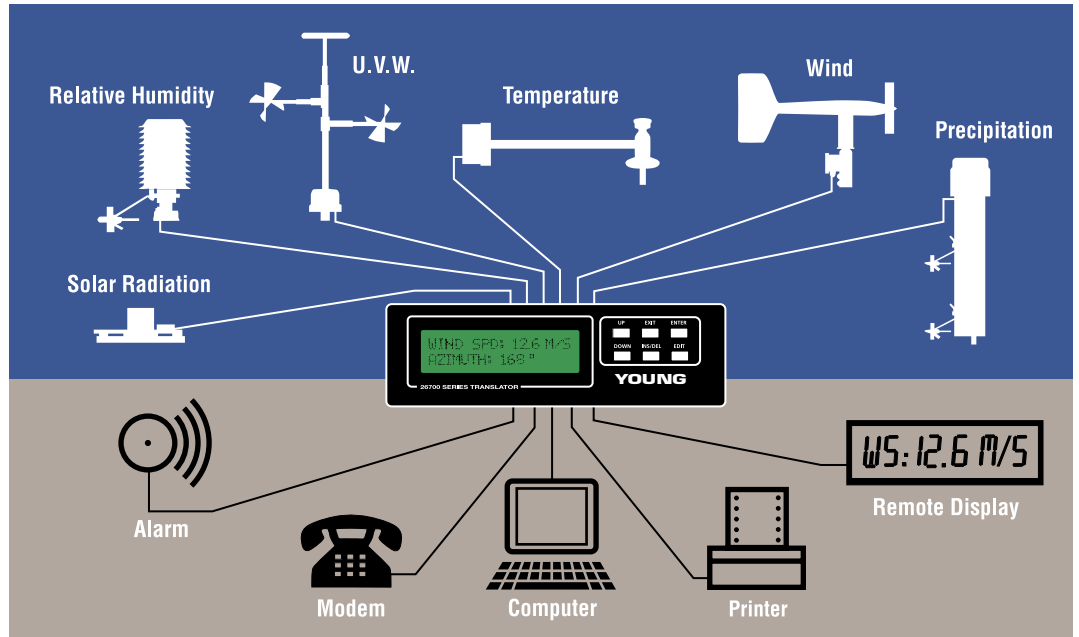
▲ The 26700 Programmable Translator accepts from most meteorological sensors and interfaces directly with many peripheral devices.
