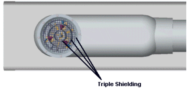
Detailed view of bottom of temperature sensor showing triple shielding, air intake, and screen.
