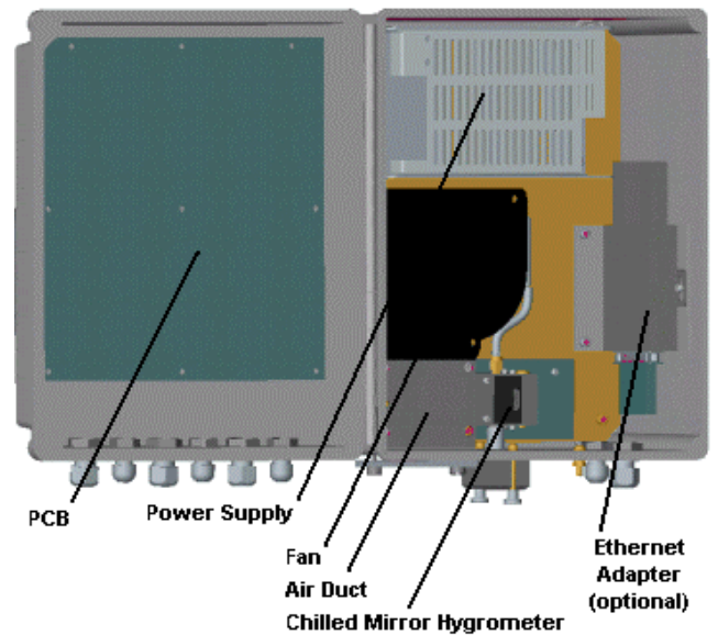
Chilled Mirror Hygrometer enclosure and instrument electronics.
