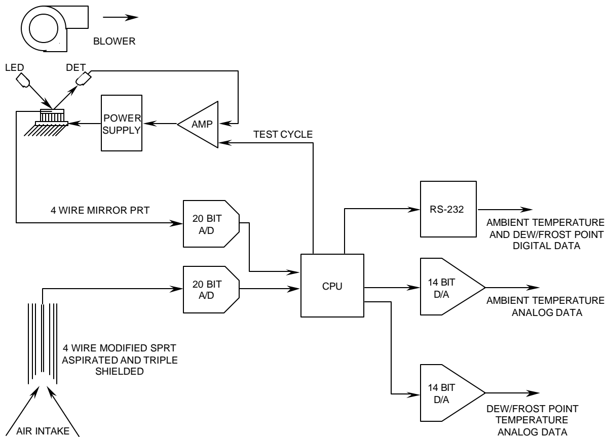
MET-2010 functional block diagram
