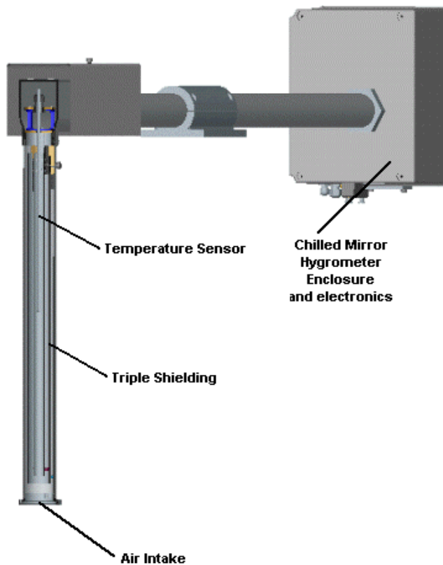
Cross section identifying temperature sensor, triple shielding, and air intake.
