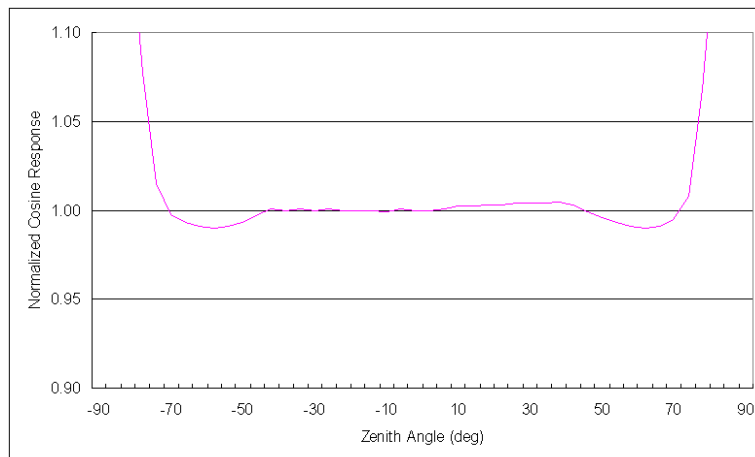
TSP-400 Cosine Response
